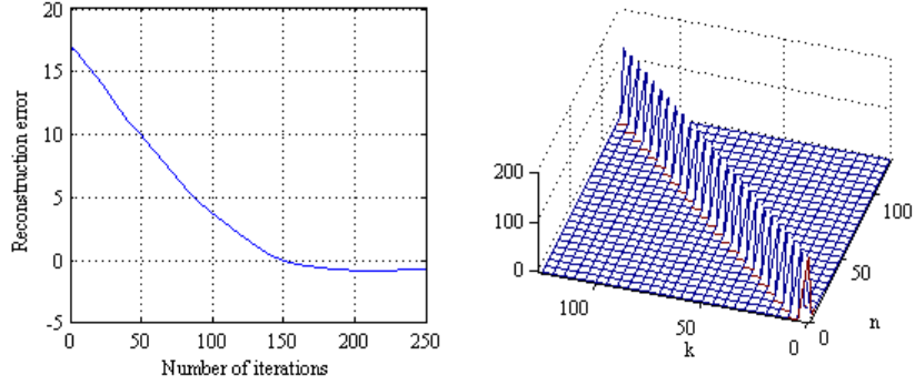
Figure 2: The reconstruction error (left) during the iterations in the case of mono-component LFM signal from Fig. 1 and the S-method of the analyzed signal (right).
