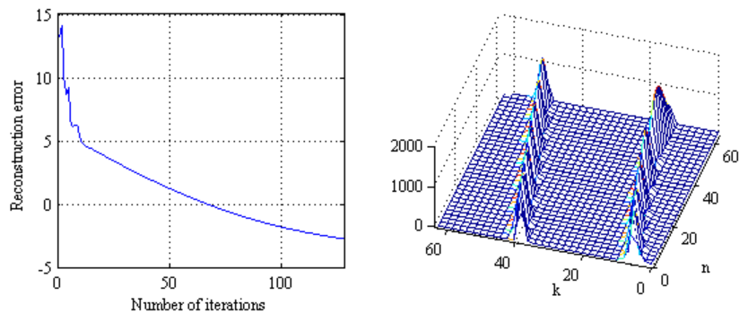
Figure 6: The reconstruction error (left) during the iterations in the case of multi-component signal shown on Fig. 5 and the corresponding S-method (right).
