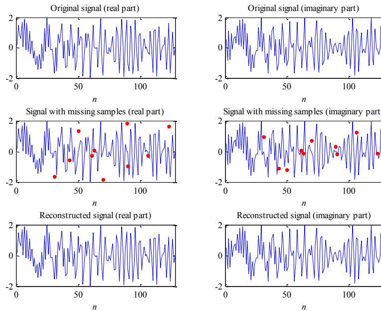
Figure 5: The reconstruction of multi-component signal with 8% of missing samples: first row shows the real and imaginary parts of the original signal; signal with missing samples is shown in the second row, where missing values are denoted with red dots; third row presents real and imaginary parts of the reconstructed signal
