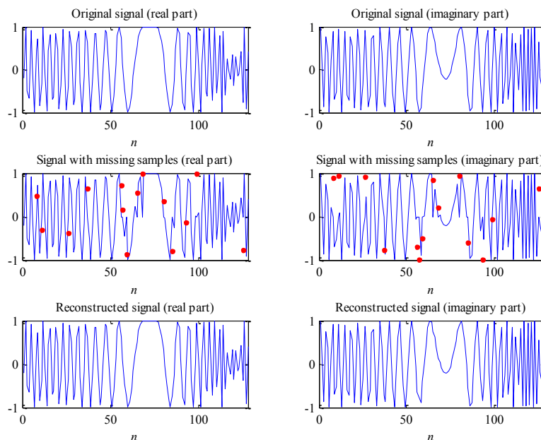
Figure 3: The reconstruction of polynomial-phase signal with 11% of missing samples: first row shows the real and imaginary parts of the original signal; signal with missing samples is shown in the second row, where missing values are denoted with red dots; third row presents real and imaginary parts of the reconstructed signal
