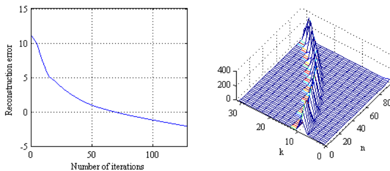
Figure 4: The reconstruction error (left) during the iterations in the case of mono-component polynomial-phase signal shown on Fig. 3 and the corresponding S-method (right).
