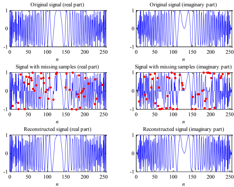
Figure 1: The reconstruction of LFM signal with 20% of missing samples: first row shows the real and imaginary parts of the original signal; signal with missing samples is shown in the second row, where missing values are denoted with red dots; third row presents real and imaginary parts of the reconstructed signal
