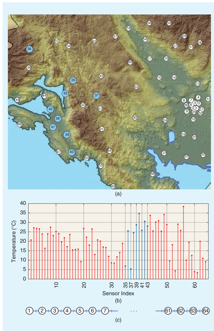
FIGURE 1. An illustration of temperature sensing as a classical signal processing problem. (a) A map of sensing locations in a geographic region along the Adriatic Sea (Montenegro). (b) Temperatures measured at N = 64 sensing locations. In standard signal processing, the spatial sensor index is used for the horizontal axis and serves as the signal domain. (c) This domain can also be interpreted as a directed path graph but lacks physical intuition as, for example, sensor 37 (mountains) is followed by sensor 38 (coast), with a drastic difference in temperature.
