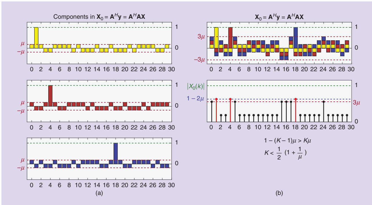
FIGURE 4. The illustration of the coherence index relation for K = 3 . (a) The components of the initial estimate, \mathbf{X}_0 = \mathbf{A}^H \mathbf{y} = \mathbf{A}^H \mathbf{A} \mathbf{X} , that result from each of the three unity-valued nonzero elements in \mathbf{X} at k \in \{1, 4, 18\} . (b) The components are combined into the initial estimate, \mathbf{X}_0 . The positions of the nonzero elements in \mathbf{X} are detected at k \in \{1, 4, 18\} using the absolute value of the initial estimate, |X_0(k)| , if their amplitudes, reduced for a maximum possible disturbance, 2\mu , from the other two components are above the maximum possible disturbance, 3\mu , of all three components at the position of an original zero-valued element in \mathbf{X} , k \notin \{1, 4, 18\} . The condition for the correct detection of the nonzero element positions with K = 3 is, therefore, 1 - 2\mu > 3\mu ; that is, 1 - (K - 1)\mu > K\mu , which generalizes to any K .
