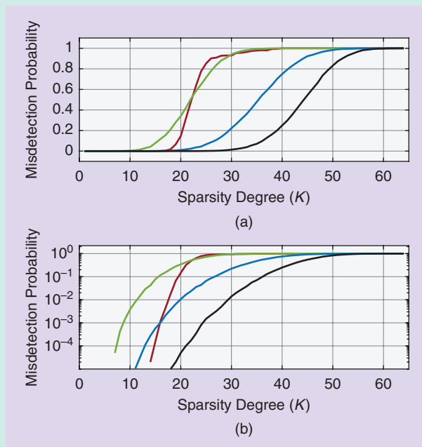
FIGURE S1. The misdetection probability of the original nonzero element positions, given in (a) linear and (b) logarithmic scales. The measurement matrix, \mathbf{A} , took the forms of ETF (red); random, partial DFT (black); random, real-valued Gaussian (green); and complex-valued Gaussian measurement (blue) matrices.
