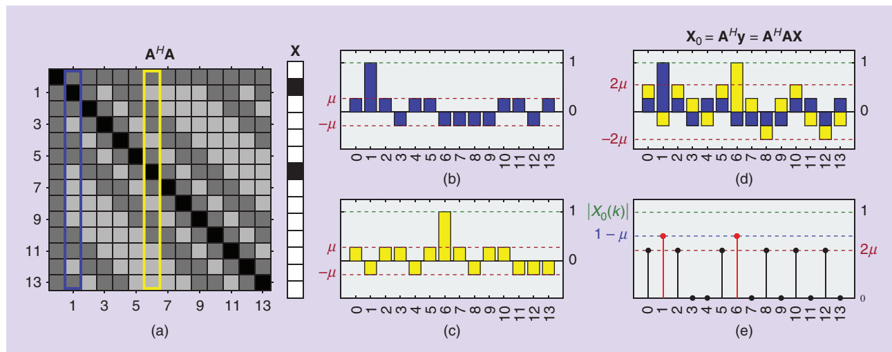
FIGURE 2. An illustration of the coherence index relation for K=2 . (a) The matrix \mathbf{A}^H \mathbf{A} for the ETF matrix \mathbf{A} from Figure 1 and the original elements in \mathbf{X} with nonzero values at k_1=1 and k_2=6 . The values in matrix \mathbf{A}^H \mathbf{A} are indicated by black equals 1, white equals 0, dark gray equals +\mu , and light gray equals -\mu . The components in the initial estimate \mathbf{X}_0 = \mathbf{A}^H \mathbf{y} , calculated using the measurements \mathbf{y} = \mathbf{A} \mathbf{X} that result from (b) the nonzero element at k_1=1 in the blue bar plot and (c) k_2=6 , in the yellow bar plot. The visual demonstration that the condition for a correct detection of the original nonzero element position from the initial estimate is 1 - \mu > 2\mu , with (d) the stacked bar plot for both components and (e) the resulting |X_0(k)| .
