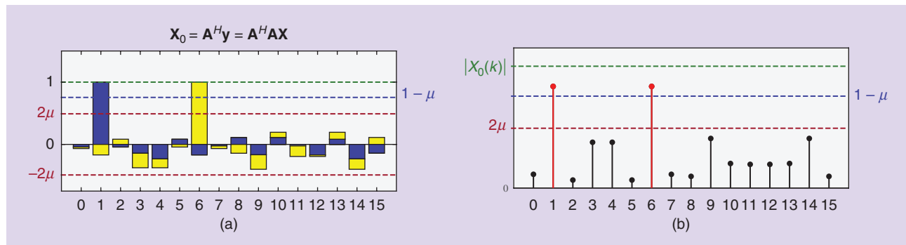
FIGURE 3. (a) The initial estimate, \mathbf{X}_0 , for a 12 \times 16 partial DFT measurement matrix, where \mu = 0.2455 , and the sparsity degree of K = 2 in \mathbf{X} , with X(1) = X(6) = 1 [the real part of X_0(k) is presented in the stacked bar plot]. (b) The positions of nonzero elements in \mathbf{X} are detected at k \in \{1, 6\} if their amplitude, when reduced by the maximum possible disturbance from the other component, \mu , is above the maximum possible disturbance, 2\mu , of both components, at a position of an original zero-valued element in \mathbf{X} , k \notin \{1, 6\} . Observe that there is a larger misdetection margin compared to the ETF case, indicated by the corresponding (1 - \mu) and 2\mu levels, that is a consequence of different distributions of disturbances (off-diagonal elements of matrix \mathbf{A}^H\mathbf{A} ).
